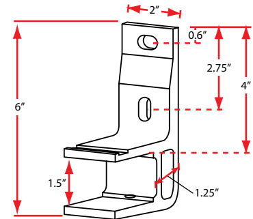
S / L series Wall Bracket
